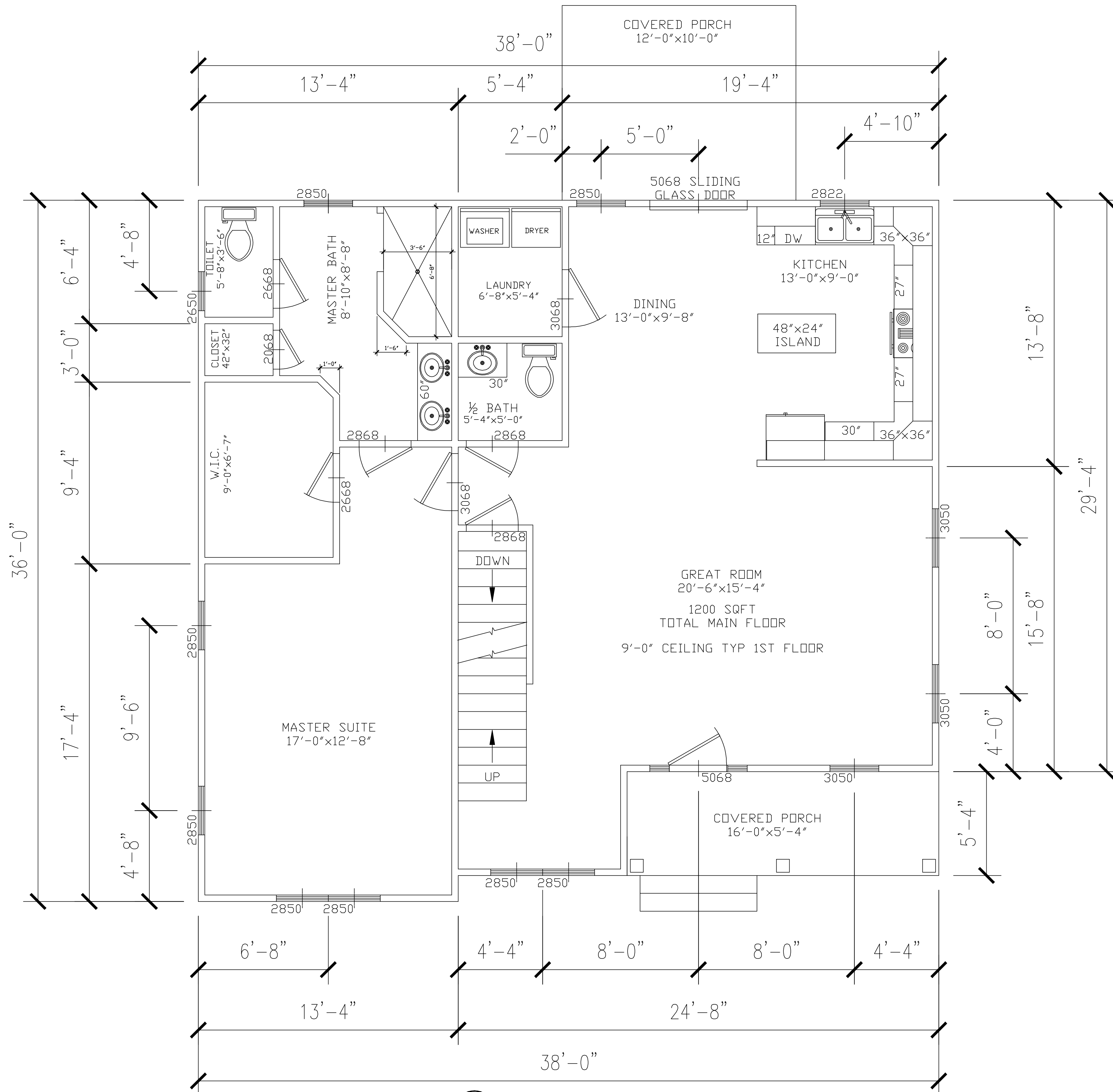
1 1st FLOOR PLAN S-1.1 SCALE: 3/8"=1'-0"
