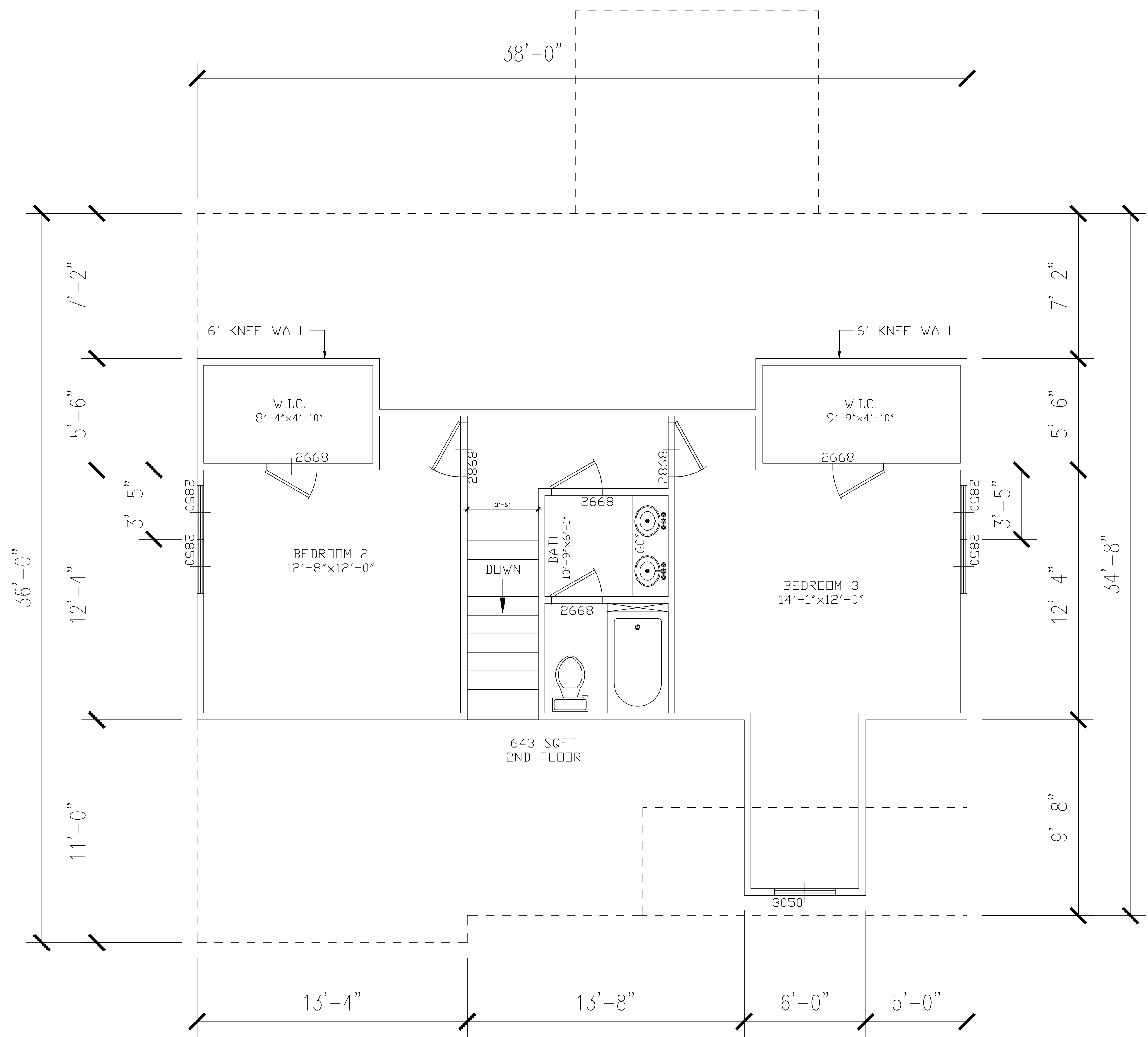
1 2ND FLOOR PLAN S-1.1 SCALE: 3/8"=1'-0"
